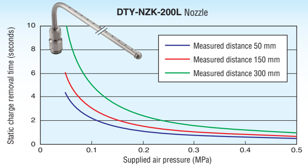
Free Mounting L-Shaped Bar Nozzle (200 mm) Static Charge Removal Characteristics
