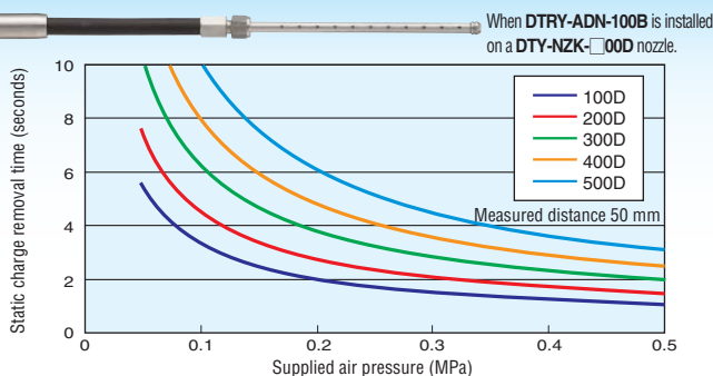
Bender Nozzle Length and Static Charge Removal Characteristics (Straight Bar Nozzle 100 mm) When DTRY-ADN-100B is installed on a DTY-NZK-□00D nozzle.
