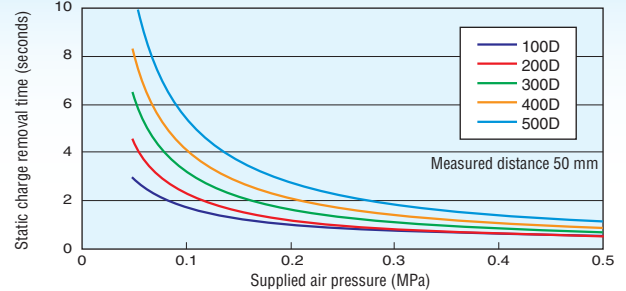
Bender Bar Nozzle Length and Static Charge Removal Characteristics (Flat Nozzle) When DTRY-ADN-FT01 is installed on a DTY-NZK-□00D nozzle.
