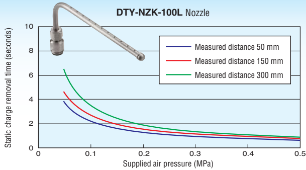
Free Mounting L-Shaped Bar Nozzle (100 mm) Static Charge Removal Characteristics
