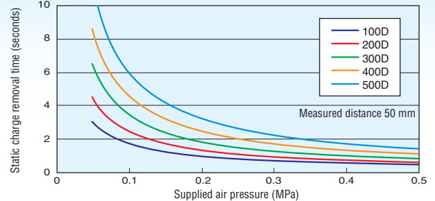
Bender Nozzle Length and Static Charge Removal Characteristics (Straight Bar Nozzle 200 mm) When DTRY-ADN-200B is installed on a DTY-NZK-□00D nozzle.
