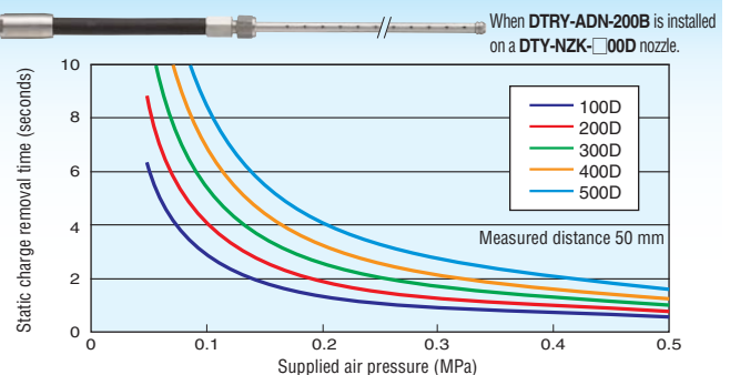
Bender Nozzle Length and Static Charge Removal Characteristics (Straight Bar Nozzle 200 mm) When DTRY-ADN-200B is installed on a DTY-NZK-□00D nozzle.
